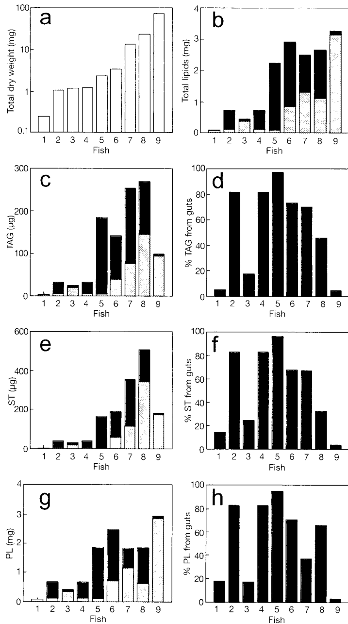
Fig. 1. (a) Total dry weight (defatted dry weight + lipids from gut contents + lipids from larval tissue); (b) total lipids; (c) triacylglycerol (TAG); (d) percentage of TAG from gut contents; (e) sterols (ST); (f) percentage of ST from gut contents; (g) phospholipids (PL); (h) percentage PL from gut contents of 9 (fish 1 to 9) cod larvae. Gut contents (solid bars) and larval tissue (cross-hatched bars) were analysed separately for lipid class composition. These 9 larvae are a representative subset of 20 larvae processed in an identical manner (see text)
