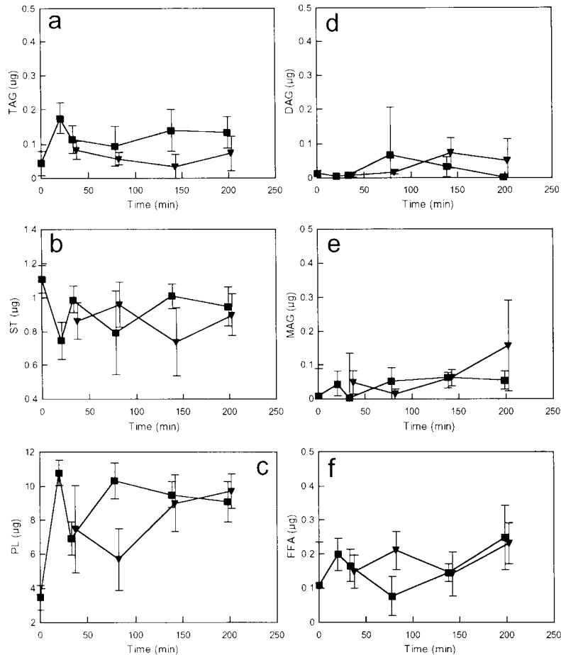
Fig. 2. Measures of individual lipid classes as a function of time delay at 2 different holding temperatures. Average ( \pm 2 SE) (a) triacylglycerols (TAG); (b) sterols (ST); (c) polar or phospholipids (PL); (d) diacylglycerols (DAG); (e) monoacylglycerols (MAG); and (f) free fatty acids (FFA) for larval cod at 3°C (■) and 21°C (▼). Larvae were collected live ( t = 0 ) and after being subjected to simulated sampling in a mesh container ( t = 20 ) at 3°C, and at several time delays after simulated sampling and prior to preservation. Data presentation at fixed intervals have been slightly offset to allow comparison of standard errors. Sample sizes ranged from 28 to 40 larvae
