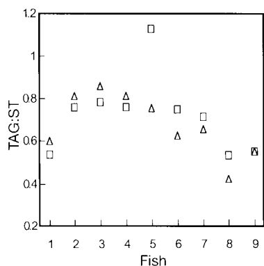
Fig. 3. Comparison of triacylglycerol to sterol ratio (TAG:ST) with lipids from gut contents included ( \Delta ) and excluded ( \square ) for 9 cod larvae representative of the 20 larvae for which guts and carcasses were analysed separately
