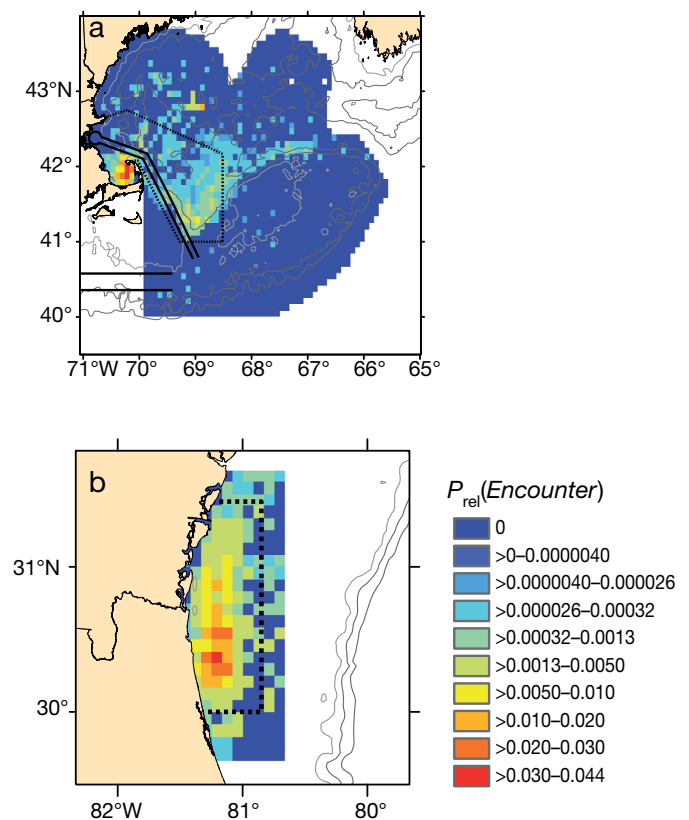
Fig. 7. Bathymetric (50, 100, 200 m) charts illustrating the relative probability of a vessel–whale encounter in (a) the Cape Cod Bay and Great South Channel habitats and in (b) the southern calving ground habitat where probabilities have been standardized for direct comparison among habitats. The mandatory ship reporting areas are outlined (dashed lines) as are the International Maritime Organization traffic separation schemes for the ports of Boston and New York (solid black lines)
